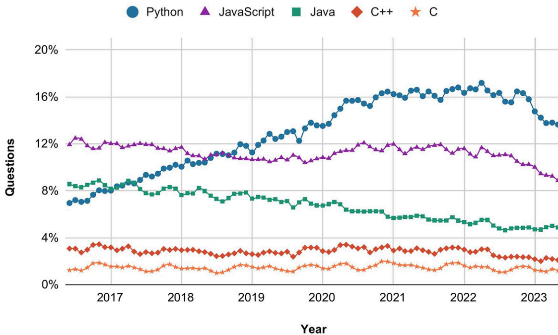
Figure 1.3 Stack Overflow questions per month. Source: data.stackexchange.com
